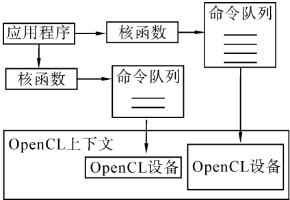
图10 OpenCL 通过命令队列和上下文管理核函数执行 Fig.10 OpenCL manages the kernels through command queue and context
